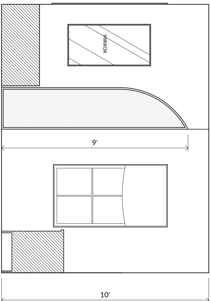
④ MICHELE'S BATH - WEST
